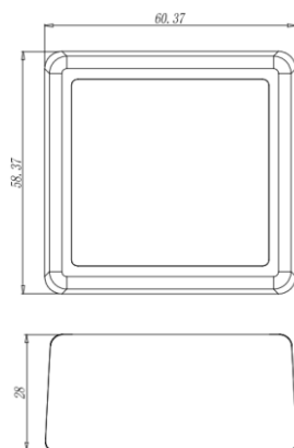
Figure 1: Dimension
