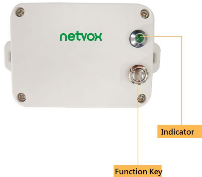
Fig.1 R718MA Appearance
